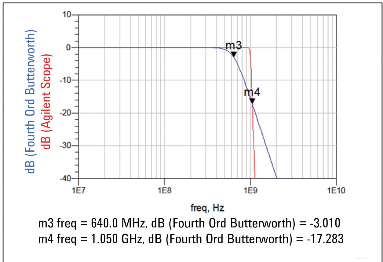
Figure 4. Frequency response of 1 GHz scope channel and fourth order Butterworth filter
