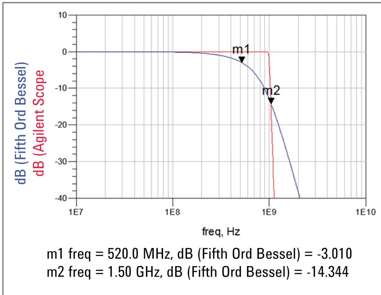
Figure 2. Frequency response of 1-GHz scope channel and fifth-order Bessel filter
