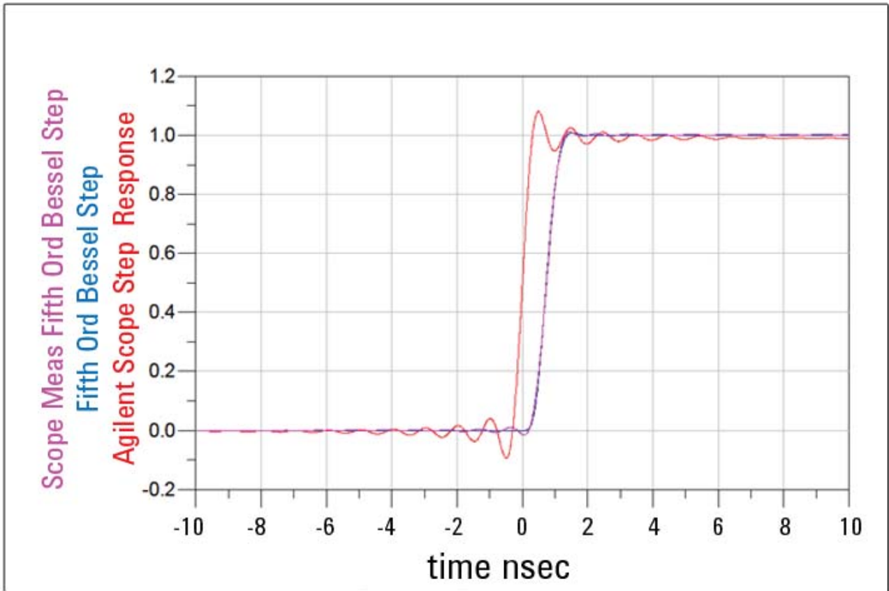
Figure 1. 1-GHz scope step response and scope measuring a step with little overshoot
