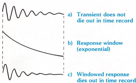
Figure 3.35 Using the response window
