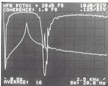
Figure 4.17 Magnitude and coherence of frequency response
