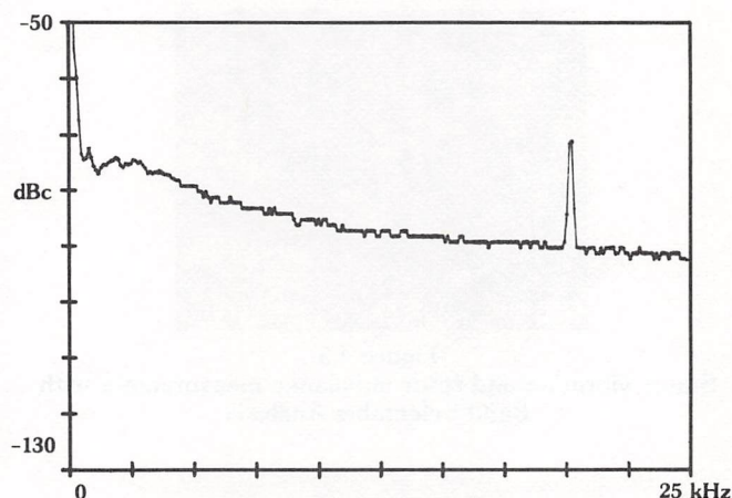
b) Phase noise of a frequency synthesizer — RMS averaging and Hanning window used for noise measurements
