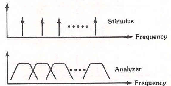
Figure 3.38 Pseudo-random noise as a stimulus
