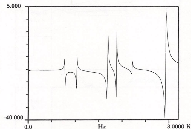
Figure 4.29 A frequency response of the plate.
