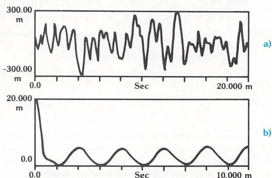
Figure 4.24 Auto correlation of a sine wave buried by noise
