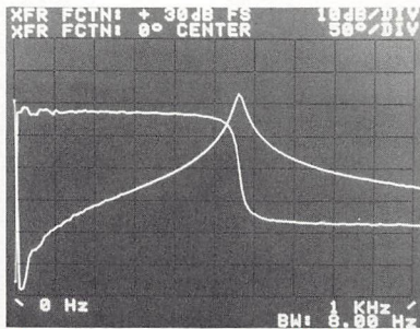
b) Frequency response magnitude and phase
