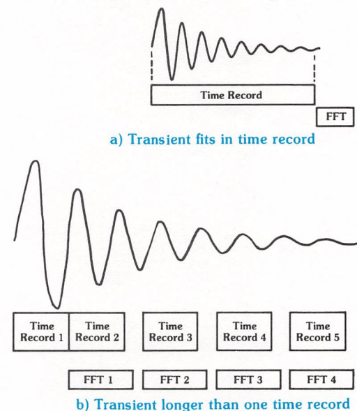
Figure 3.50 Transient analysis
