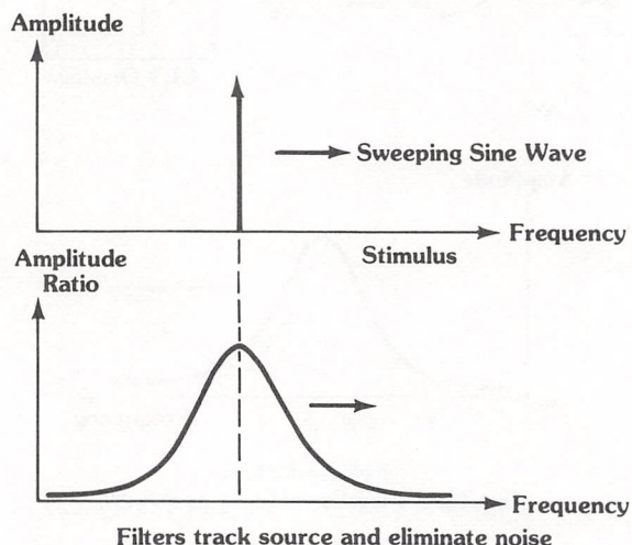
Figure 2.26 Tuned network analyzer operation
