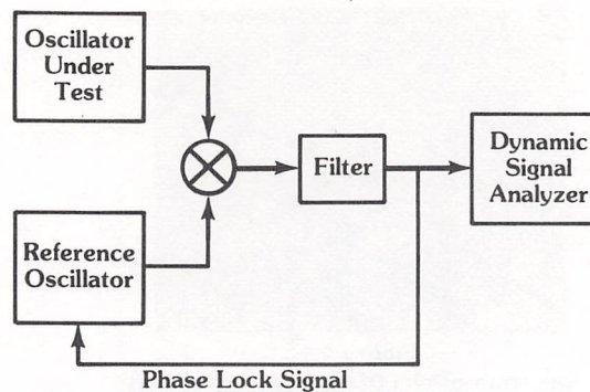
a) Block diagram of phase noise measurement
