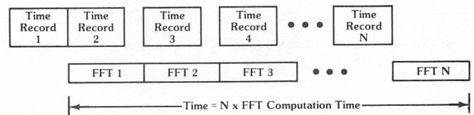
Figure 3.49 RMS averaging time
