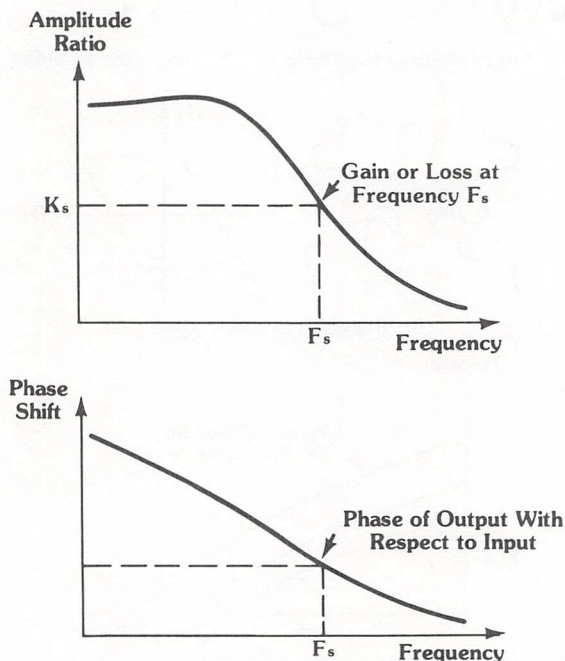
Figure 2.18 The frequency response of a network
