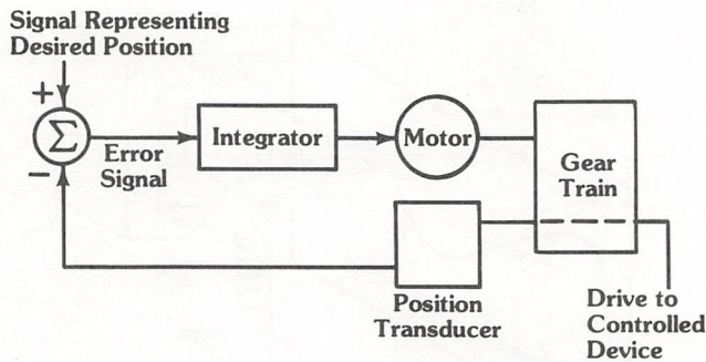
Figure 2.16 A positioning system
