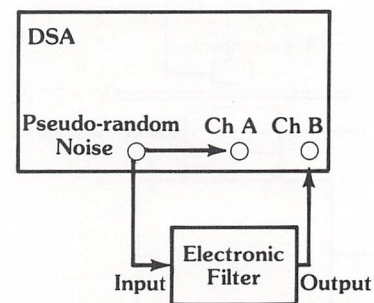
Figure 4.9 Test setup to measure frequency response of filter.
