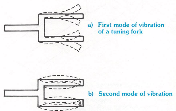
Figure 2.28 Example vibration modes of a tuning fork
