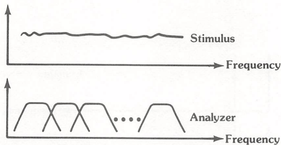
Figure 3.39 Random noise as a stimulus
