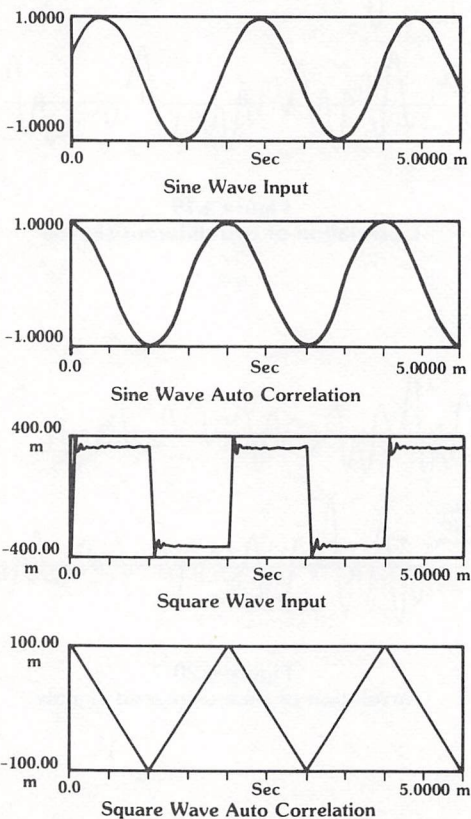
Figure 4.23 Auto correlation of periodic waveforms
