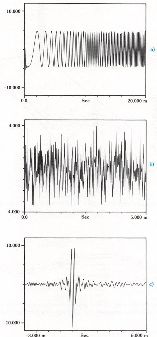
Figure 4.25 Simulated radar cross correlation
