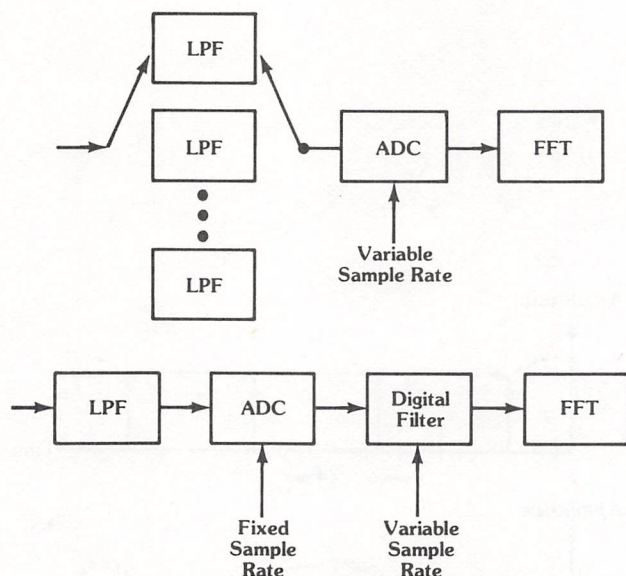
Figure 3.19 Block diagrams of analog and digital filtering
