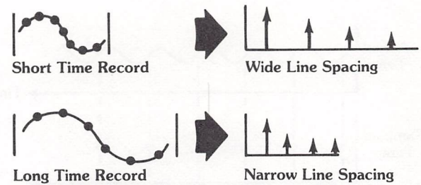
Figure 3.9 Frequency range of Dynamic Signal Analyzers is determined by sample rate
