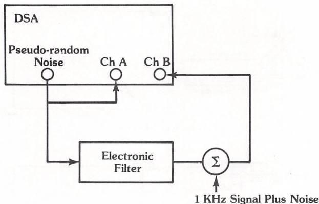
Figure 4.15 Simulation of frequency response measurement in the presence of noise.
