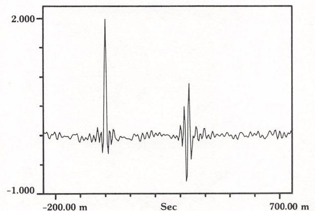
Figure 4.26 Cross correlation shows multiple transmission paths.
