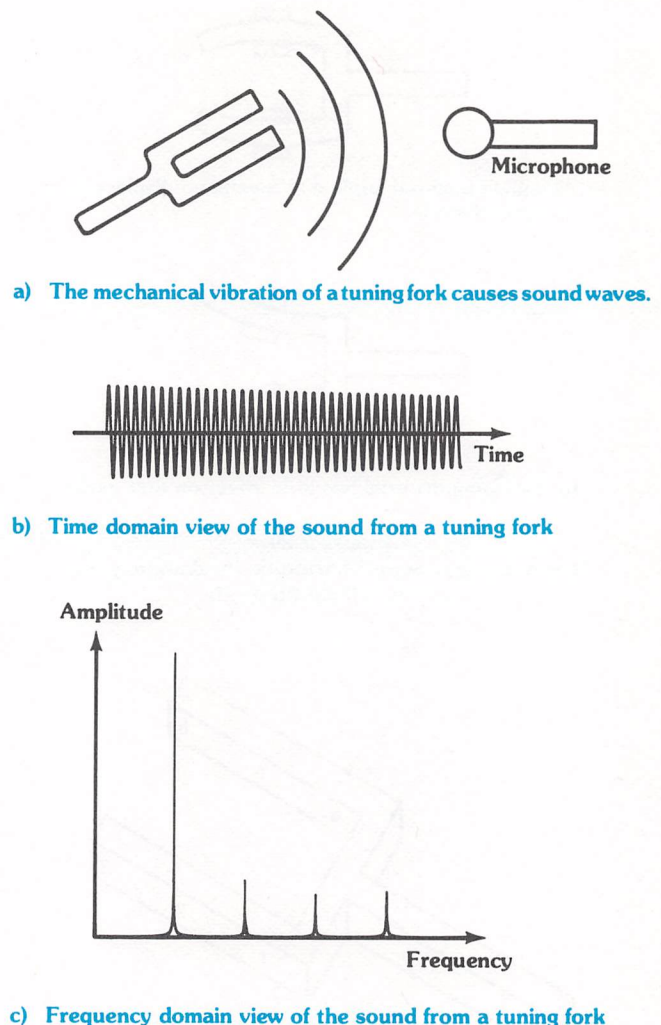
Figure 2.27 The vibration of a tuning fork
