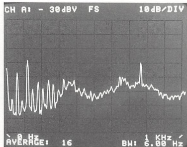
Figure 4.4 Spectrum of electrical motor vibration
