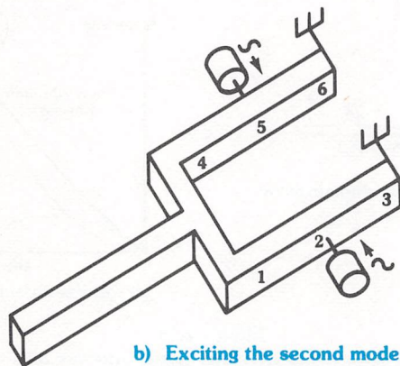
Figure 2.33 Single mode excitation modal analysis
