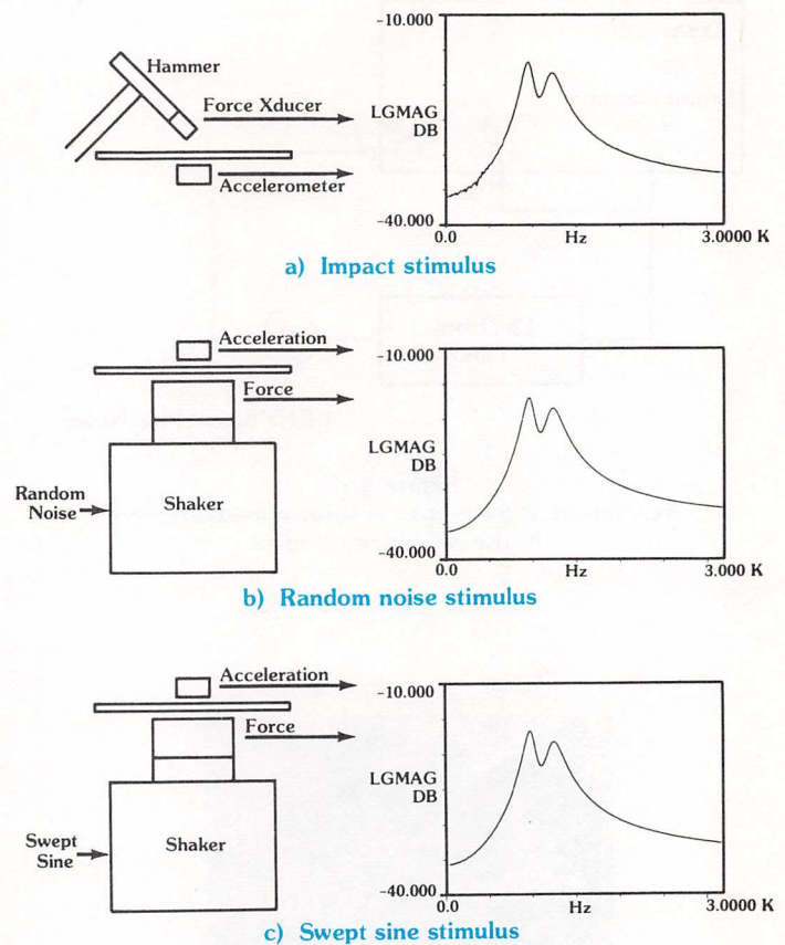
Figure 4.12 Frequency response of a linear network is independent of the stimulus used.
