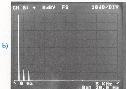
a) & b) Sine wave periodic in time record
