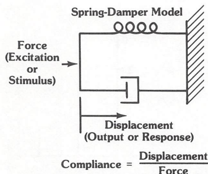
b) Compliance of a shock mount
