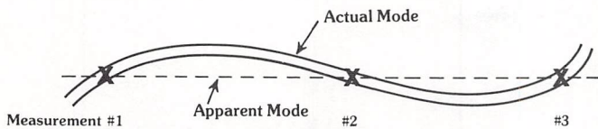
Figure 4.28 Spatial Aliasing — Too few measurement points lead to inaccurate analysis of high frequency bending mode.
