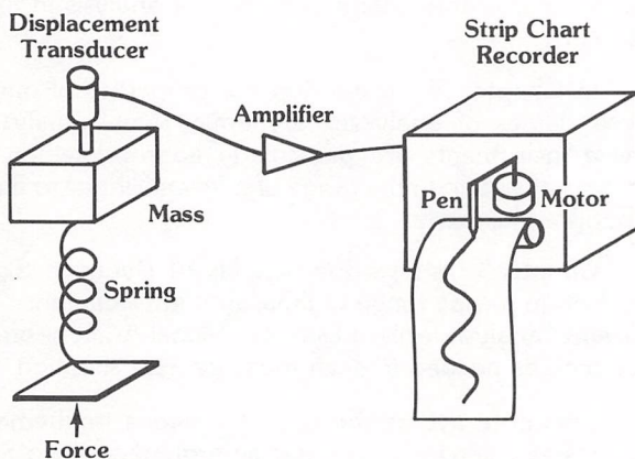
Figure 2.2 Indirect recording of displacement
