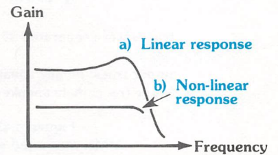
Figure 3.42 Non-linear system
