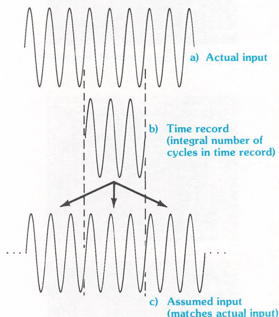
Figure 3.23 Input signal periodic in time record
