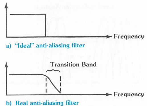
Figure 3.18 Actual anti-alias filters require higher sampling frequencies.
