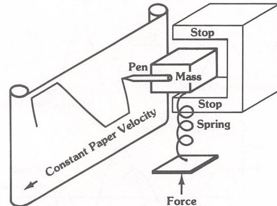
b) System is non-linear for large deflections
