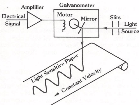
Figure 2.3 Simplified oscillograph operation
