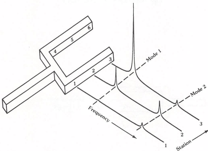
b) Frequency response at measurement points
