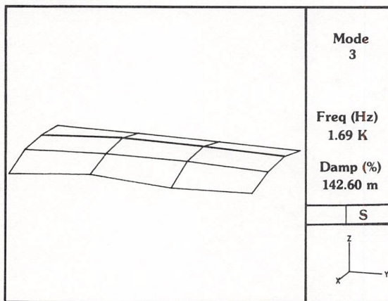
Figure 4.30 Mode shapes of a rectangular plate.
