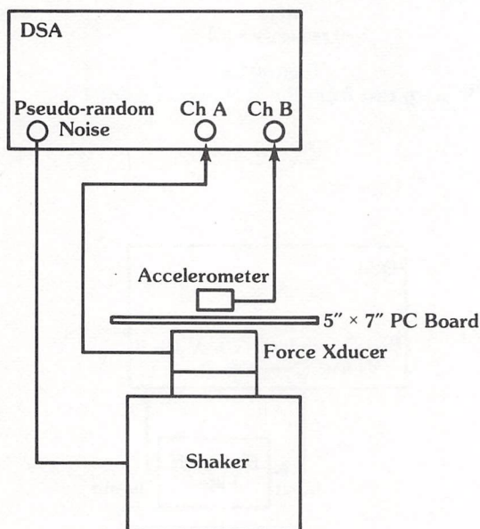
Figure 4.11 Frequency response test of a mechanical structure.
