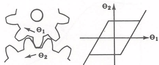
b) Backlash in a gear train
