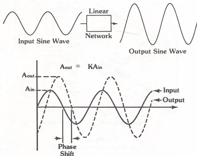
Figure 2.17 Linear network response to a sine wave input
