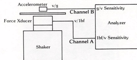
Figure 4.13 Engineering units set input sensitivities to properly scale results.
