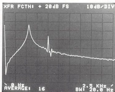
Figure 4.16 Magnitude of frequency response
