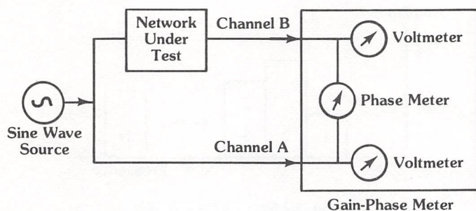
Figure 2.25 Gain-phase meter operation
