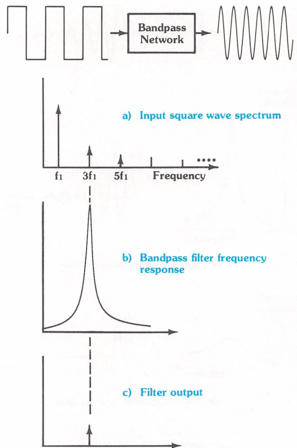
Figure 2.20 Bandpass filter response to a square wave input
