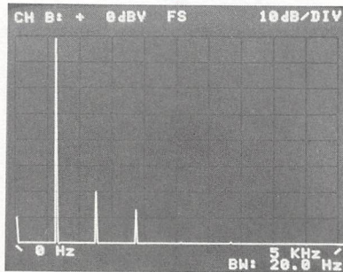
b) Frequency Domain - Small signal easily resolved
