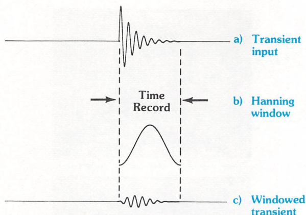
Figure 3.29 Windowing loses information from transient events.
