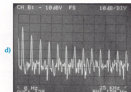
c) & d) 128 Linear averages
