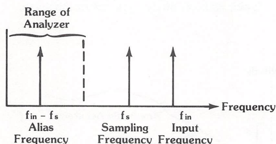
Figure 3.15 The problem of aliasing viewed in the frequency domain
