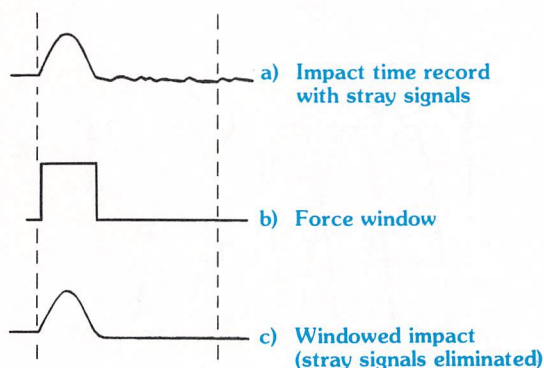
Figure 3.36 Using the force window
