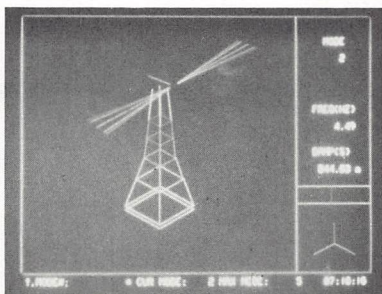
Figure 2.34 Measured mode shape
