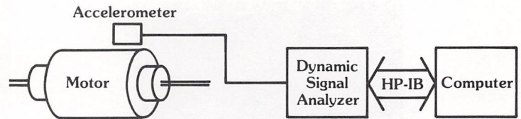
Figure 4.7 Desktop computer system for monitoring rotating machinery vibration
