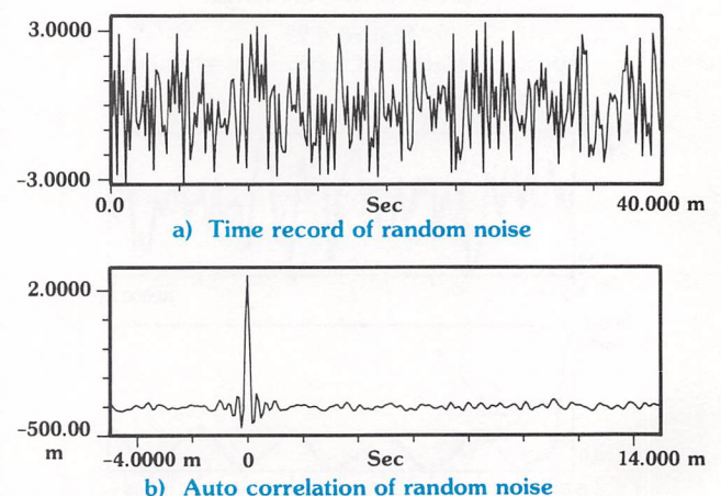
Figure 4.21 Auto correlation of random noise
