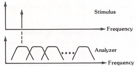
Figure 3.37 Frequency response measurements with a sine wave stimulus
