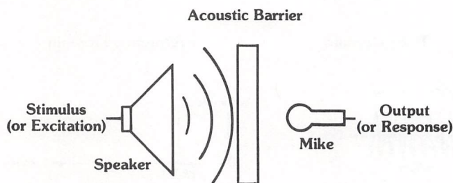
a) Sound transmission through a barrier
