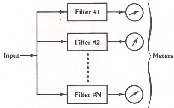
a) Simplified parallel filter analyzer
