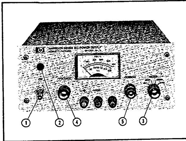
Figure 3-1. Front Panel Controls and Indicators
