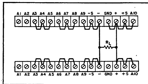
Figure 3-10. Normal Parallel
