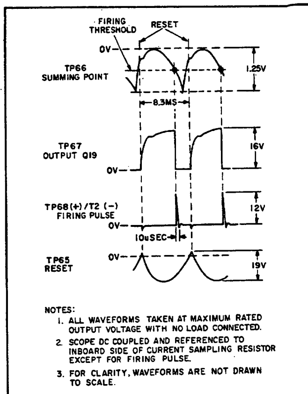
Figure 4-4. Preregulator Control Circuit Waveforms
