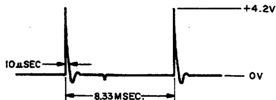
TEST POINTS 68-(T2-4)
