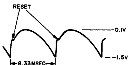
TEST POINTS 66-23 (FULL LOAD)
