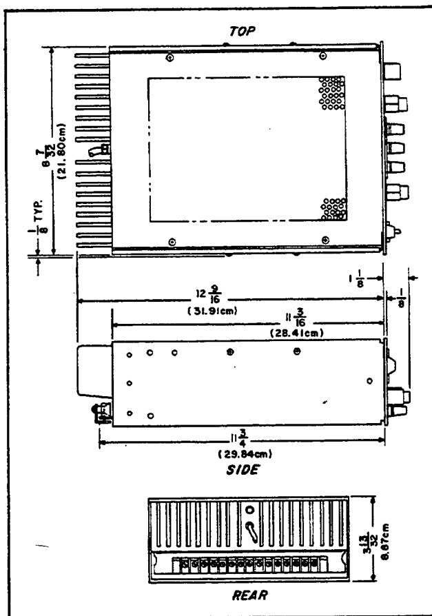
Figure 2-1. Outline Diagram
