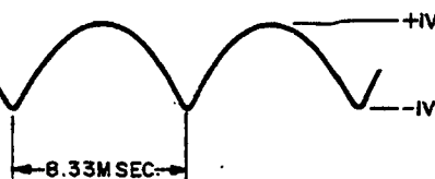
TEST POINTS 66-23 (NO LOAD, 10V OUTPUT)
