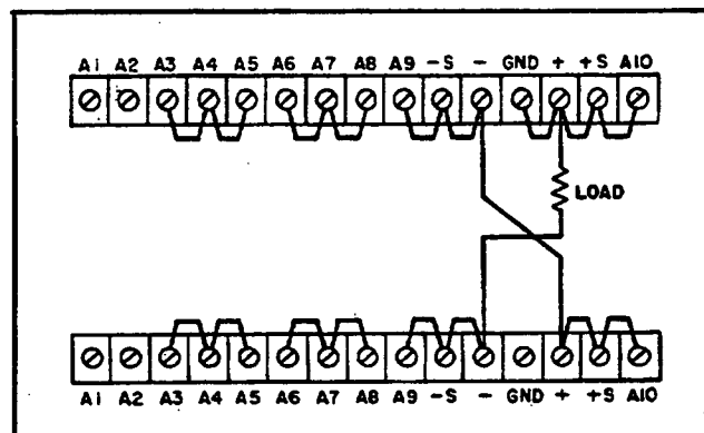
Figure 3-8. Normal Series
