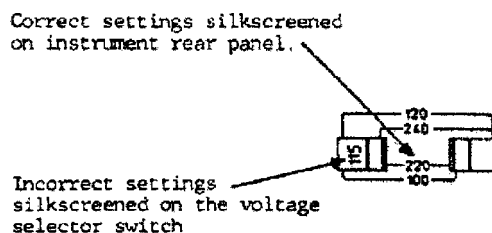
Figure 1. AC Line Voltage Switch Positions
