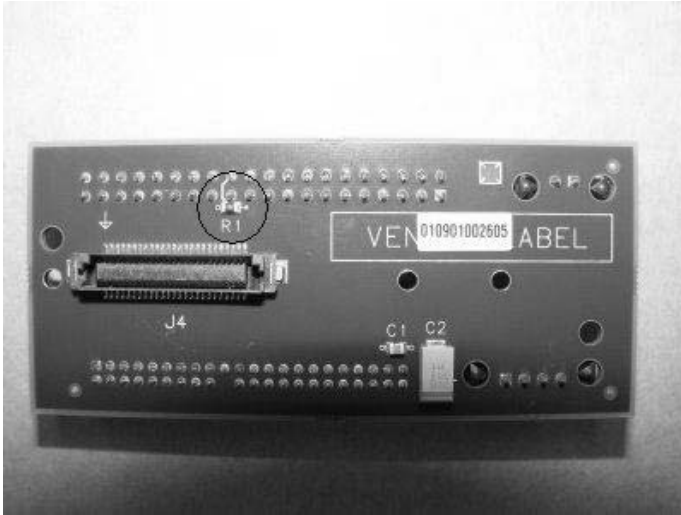
Figure 1 – Location of R1 (0 ohm resistor) on A15 CD ROM Adapter Assembly
