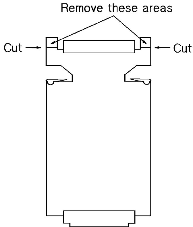
PN 08751-66594 Extender Board
